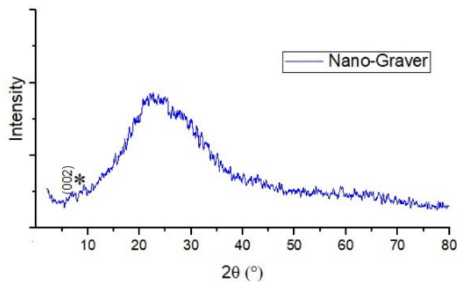
FIGURE 6. XRD characterization result of Nano-Graver material.
